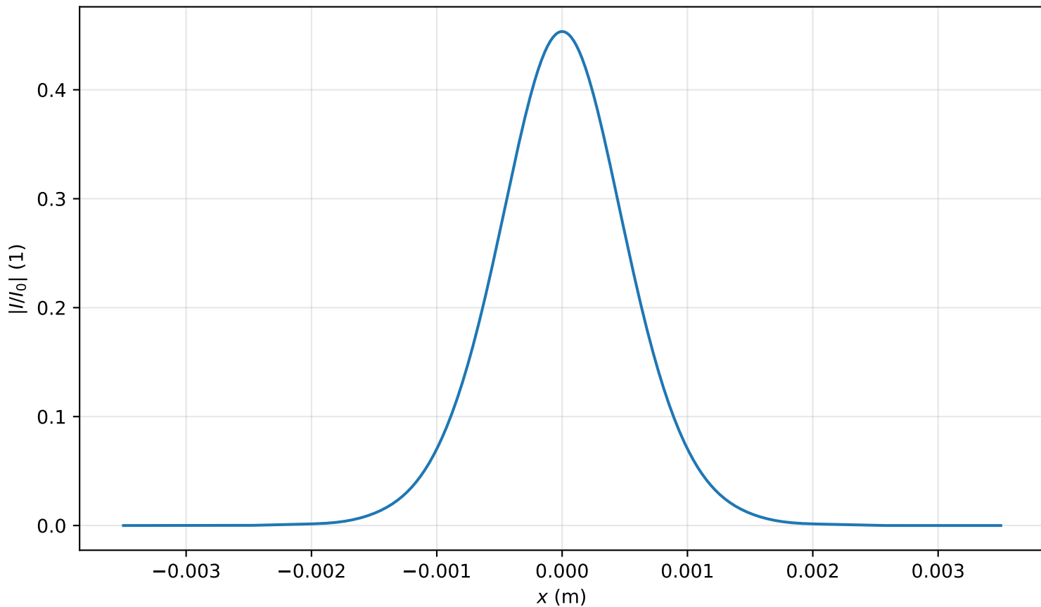
Intensity profile I(x, y = 0, z = 3.582m)/I_0 , P_{in}=0.5P_{cr} , artificial time
